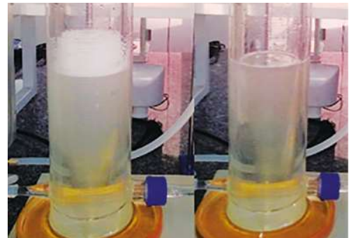
Left : foaming Right : use of Serade Antifoam
